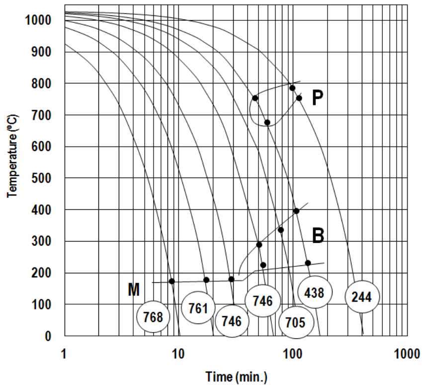
CCT Curve
